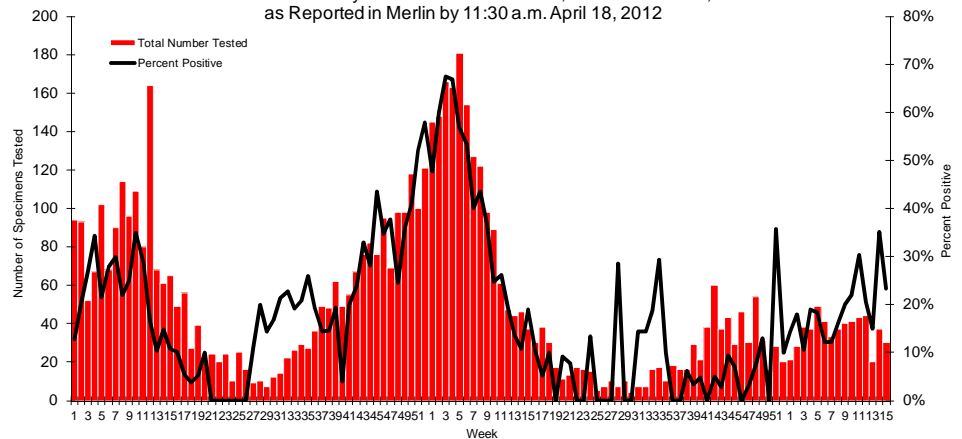
Figure 14: Number of Specimens Tested by Florida Bureau of Laboratories (BOL) and Percent Positive for Influenza by Lab EventDate* Week 1, 2010 to Week 15, 2012 as Reported in Merlin by 11:30 a.m. April 18, 2012
