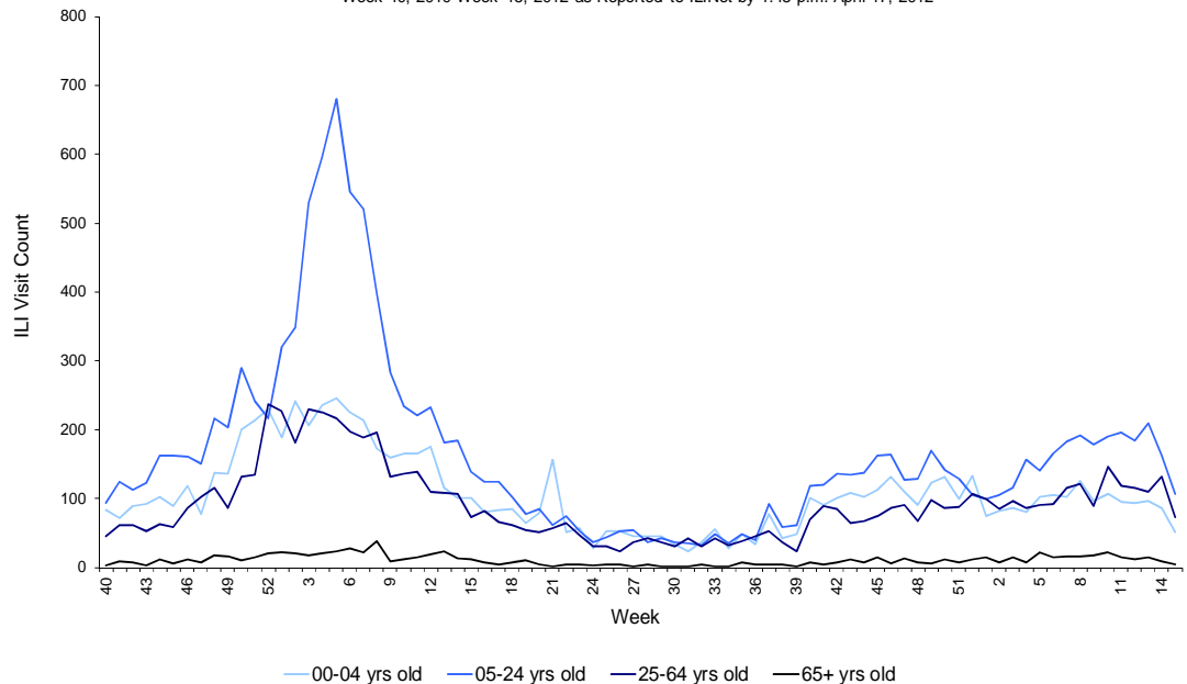
FIGURE 2: Influenza-like Illness (ILI) Visit Counts Reported by ILINet Sentinel Providers Statewide by Age Group Week 40, 2010-Week 15, 2012 as Reported to ILINet by 1:45 p.m. April 17, 2012
