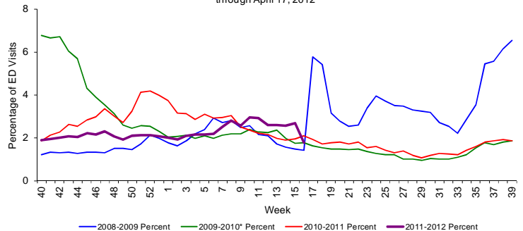
Figure 12: Percentage of Influenza-Like Illness from Emergency Department (ED) Chief Complaints, RDSTF Region 7 ESSENCE Participating Hospitals (N=48), Week 40, 2008 through April 17, 2012
