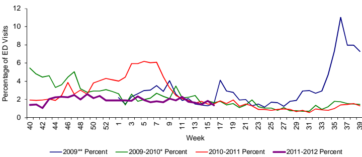
Figure 9: Percentage of Influenza-Like Illness from Emergency Department (ED) Chief Complaints, RDSTF Region 4 ESSENCE Participating Hospitals (N=31), Week 40, 2008 through April 17, 2012
