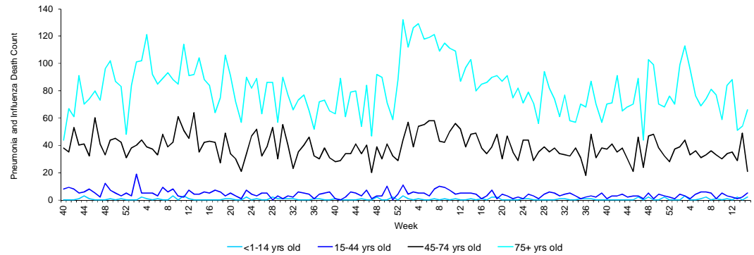
FIGURE 27: Pneumonia and Influenza Deaths in Four Age Groups for 24 Florida Counties, Week 40, 2009-Week 15, 2011 as Reported to FPIMSS by 5:00 p.m. April 14, 2012
