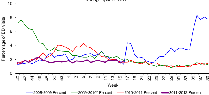
Figure 11: Percentage of Influenza-Like Illness from Emergency Department (ED) Chief Complaints, RDSTF Region 6 ESSENCE Participating Hospitals (N=15), Week 40, 2008 through April 17, 2012
