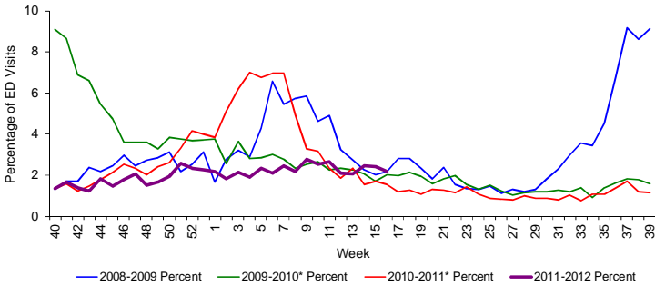
Figure 6: Percentage of Influenza-Like Illness from Emergency Department (ED) Chief Complaints, RDSTF Region 1 ESSENCE Participating Hospitals (N=5), Week 40, 2008 through April 17, 2012
