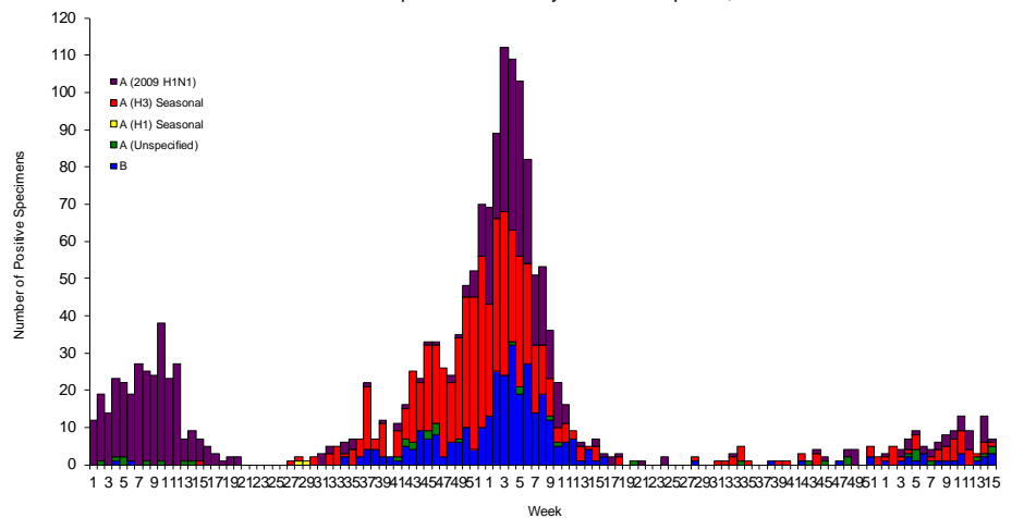
Figure 13: Number of Influenza-Positive Specimens Tested by the Florida Bureau of Laboratories (BOL) by Subtype by Lab EventDate* Week 1, 2010 to Week 15, 2012 as Reported in Merlin by 11:30 a.m. April 18, 2012
