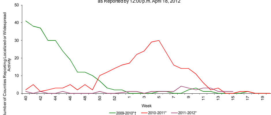
FIGURE 15: Number of Counties Reporting Moderate (Localized) or Widespread Activity, 2009-2010 (Weeks 40-20), 2010-2011 (Weeks 40-20), and 2011-2012 (Weeks 40-15) as Reported by 12:00 p.m. April 18, 2012
