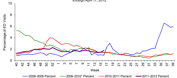
Figure 10: Percentage of Influenza-Like Illness from Emergency Department (ED) Chief Complaints, RDSTF Region 5 ESSENCE Participating Hospitals (N=49), Week 40, 2008 through April 17, 2012
