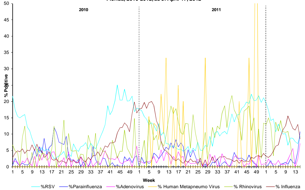
Figure 28: Percentage of Positive Respiratory Virus Tests as Collected by NREVSS, Florida, 2010-2012, as of April 17, 2012
