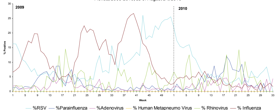
Figure 1: Percentage of Positive Respiratory Virus Tests as Collected by NREVSS, Florida, 2008-2010, as of August 24, 2010
