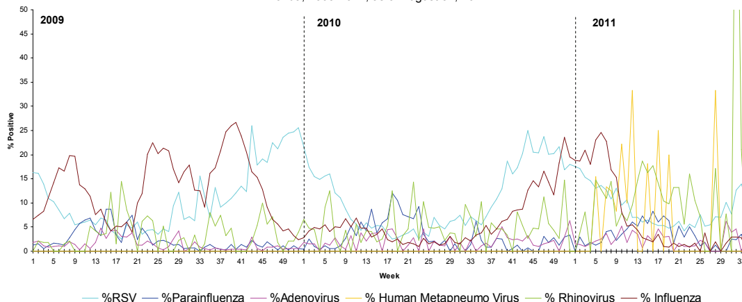
Figure 1: Percentage of Positive Respiratory Virus Tests as Collected by NREVSS, Florida, 2009-2011, as of August 31, 2011
